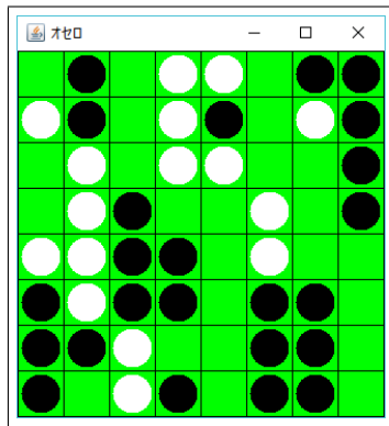
Othello.java
